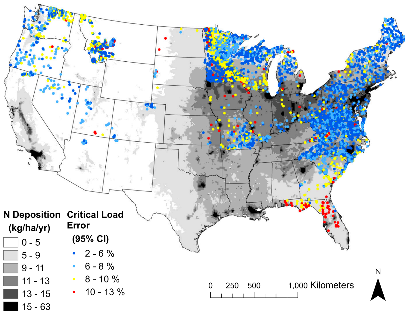
Fig. S3. Uncertainty in the critical loads for nitrogen deposition. The percent error in the critical load for each site in Fig. 2 is calculated at each site as the average of the absolute values of the lower and upper endpoints (equivalent to a plus/minus percent error for a symmetric CI) of the 95% confidence interval of 10,000 Monte Carlo simulations of coefficient uncertainty at each site. Background deposition values are the average of 27 y of wet deposition (NADP 1985–2011) plus the average of 10 y of dry deposition (CMAQ 2002–2011).
