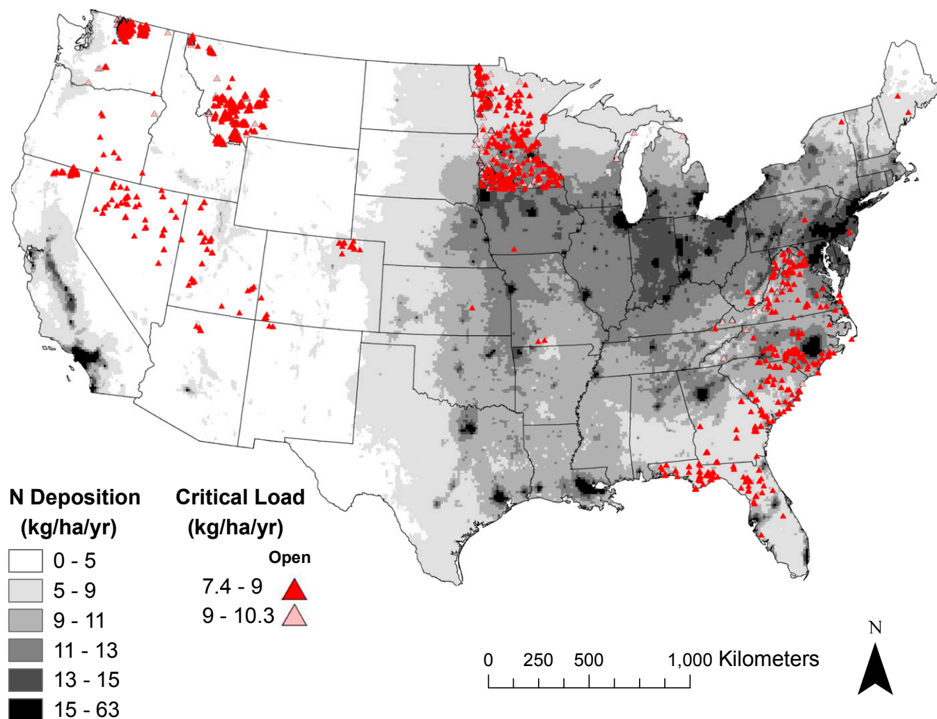
Fig. S2. Critical loads for N deposition at open vegetation sites only, based on total graminoid plus forb species richness. This figure is the same as Fig. 2, except that only the 3,317 open vegetation sites (combined grassland, shrubland, and woodland vegetation types) are portrayed here, so that those sites and the underlying N deposition can be seen more clearly. Background deposition values are the average of 27 y of wet deposition (NADP 1985–2011) plus the average of 10 y of dry deposition (CMAQ 2002–2011).
