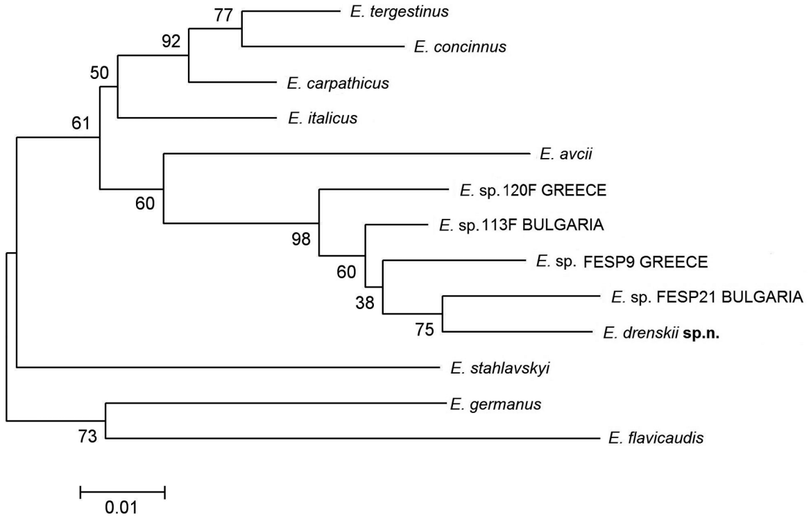
Fig. 21: A phylogenetic tree of Euscorpis based on 16S rRNA mtDNA marker. See Methods and material for explanations.
