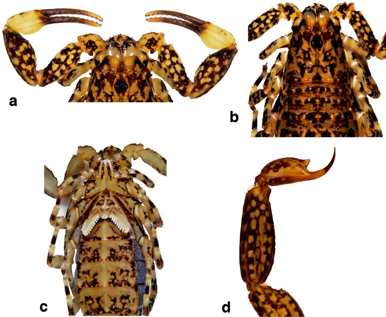
Figure 2: Female holotype of Microtityus (Parvabsonus) borincanus , sp. n.: a) pedipalps; b) carapace and anterior tergites; c) sternopectinal region and anterior sternites; d) metasomal segment V and telson, lateral view.
