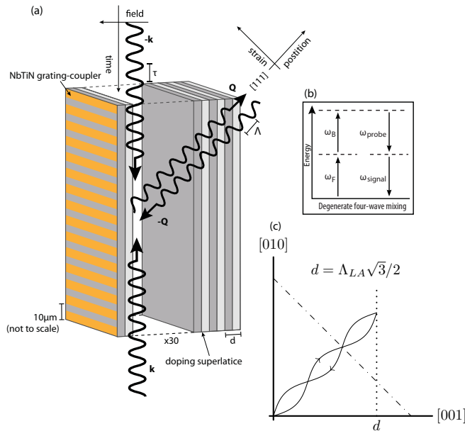
FIG. 1. (a) Schematic diagram of MAPPO showing k/-k evanescent electromagnetic fields, and (111) -directed Q/-Q (PC) acoustic fields. (b) Energy conservation diagram for D4WM. (c) Distributed-feedback phase matching, projected onto (100) plane, results in a standing LA wave (solid lines) for Q/-Q . DSL (dotted line) of period d . Gain grating (dashed-dotted line) shown. LA wavelength: \Lambda_{LA} .
