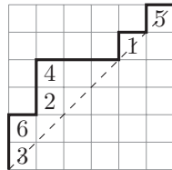
Figure 1: A labeled Dyck path from (0, 0) to (6, 6) .
